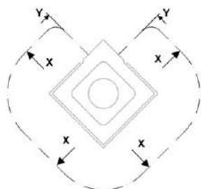
Fig. 10: Space in front of the fireplace
