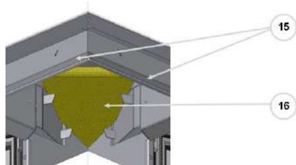
Fig. 5: Deflector in smoke hopper
