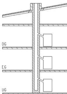
Fig. 9: Several fireplaces connected to the same chimney
