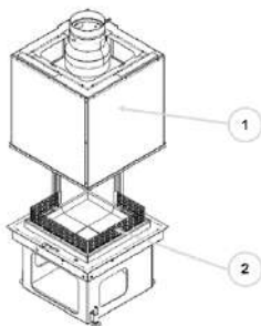
Fig. 68: Cladding and fireclay bricks
