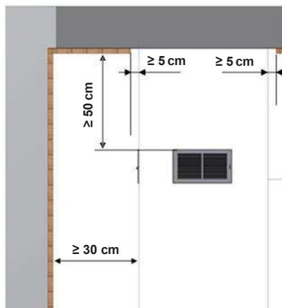
Fig. 11: Safety distances at hot air outlet
