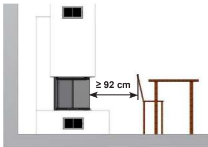
Fig. 12: Safety distances in radiant heating zone
