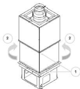
Fig. 65: Swing open the door on both sides
